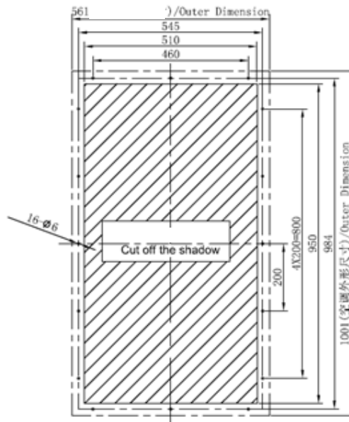
Figure 1-Cabinet Door Cutting Dimension
